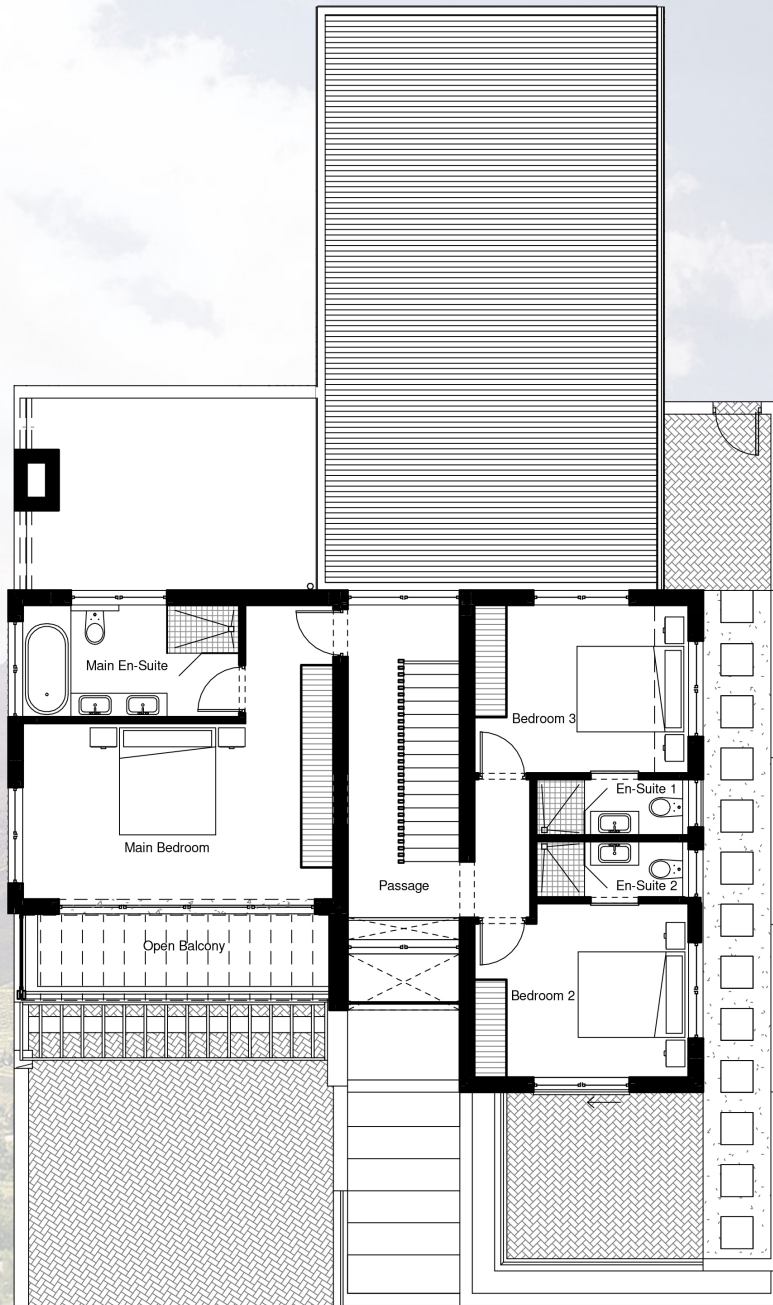
FIRST STOREY PLAN SCALE 1:100
